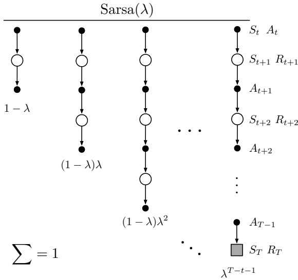
Figure 12.9: \text{Sarsa}(\lambda) 's backup diagram. Compare with Figure 12.1.
