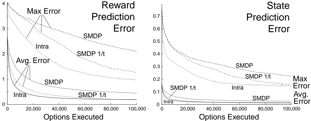
Fig. 9. Model learning by SMDP and intra-option methods. Shown are the average and maximum over \mathcal{I} of the absolute errors between the learned and true models, averaged over the eight hallway options and 30 repetitions of the whole experiment. The lines labeled ‘SMDP 1/t’ are for the SMDP method using sample averages; all the others used \alpha = 1/4 .
