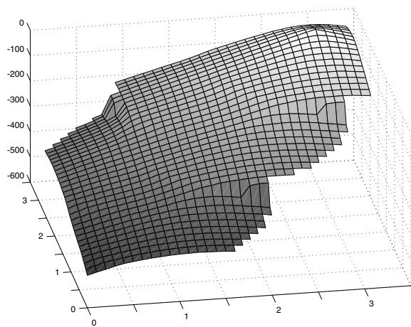
V^{\mu^I} - Values with Interruption
