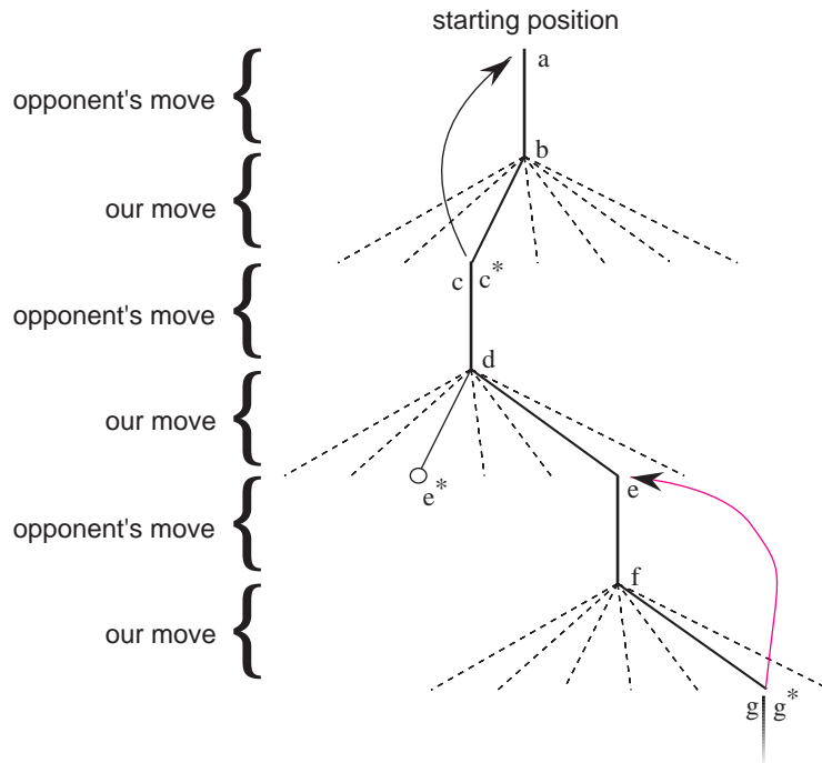
Figure 1: A sequence of tic-tac-toe moves. The solid lines represent the moves taken during a game; the dashed lines represent moves that we (our reinforcement learning player) considered but did not make. Our second move was an exploratory move, meaning that it was taken even though another sibling move, the one leading to e^* , was ranked higher. Exploratory moves do not result in any learning, but each of our other moves does, causing backups as suggested by the curved arrows and detailed in the text.
