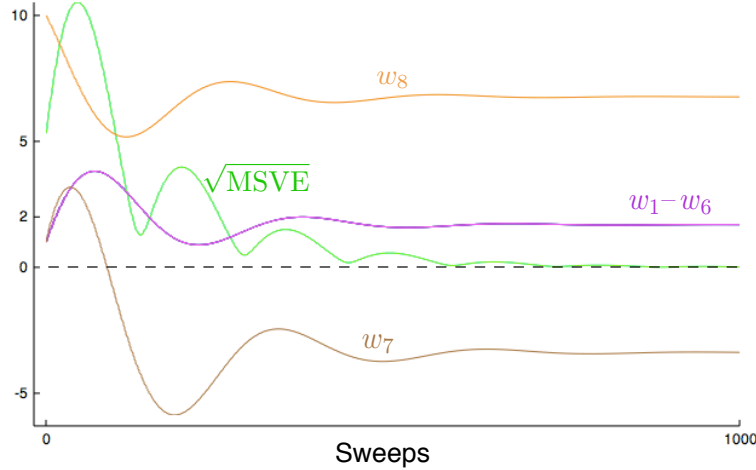
Figure 11.7: The behavior of the ETD algorithm in expectation on Baird's counterexample. The step size was \alpha = 0.03 .
