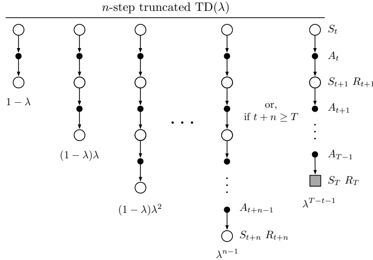
Figure 12.7: The backup diagram for truncated \text{TD}(\lambda) .
