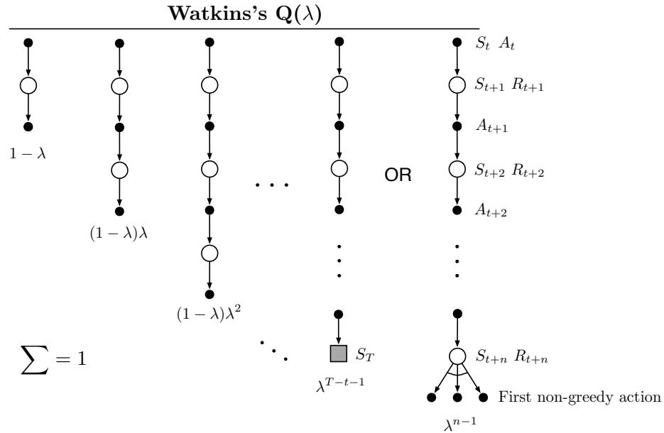
Figure 12.12: The backup diagram for Watkins's Q(\lambda) . The series of component backups ends either with the end of the episode or with the first nongreedy action, whichever comes first.
