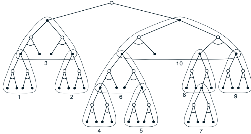
Figure 8.12: The deep backups of heuristic search can be implemented as a sequence of one-step backups (shown here outlined). The ordering shown is for a selective depth-first search.
