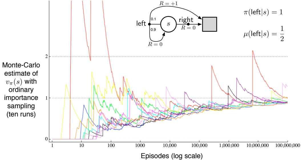
Figure 5.5: Ordinary importance sampling produces surprisingly unstable estimates on the one-state MDP shown inset (Example 5.5). The correct estimate here is 1 ( \gamma = 1 ), and, even though this is the expected value of a sample return (after importance sampling), the variance of the samples is infinite, and the estimates do not convergence to this value. These results are for off-policy first-visit MC.
