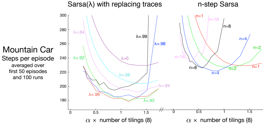
Figure 12.10: Early performance on the Mountain Car task of \text{Sarsa}(\lambda) with replacing traces and n -step Sarsa (copied from Figure 10.4) as a function of the step size, \alpha . ■
