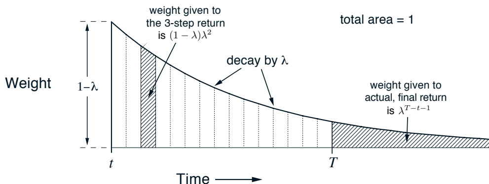
Figure 12.2: Weighting given in the \lambda -return to each of the n -step returns.
