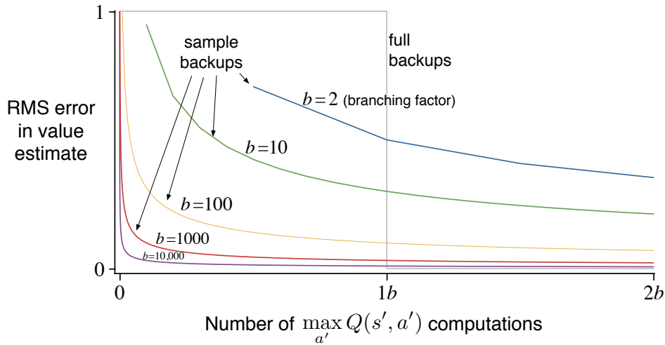
Figure 8.10: Comparison of efficiency of full and sample backups.
