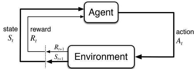
Figure 3.1: The agent–environment interaction in reinforcement learning.
