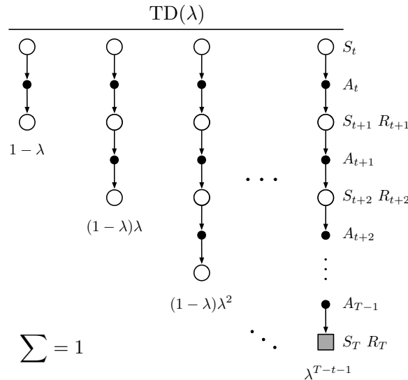
Figure 12.1: The backup digram for TD( \lambda ). If \lambda = 0 , then the overall backup reduces to its first component, the one-step TD backup, whereas if \lambda = 1 , then the overall backup reduces to its last component, the Monte Carlo backup.
