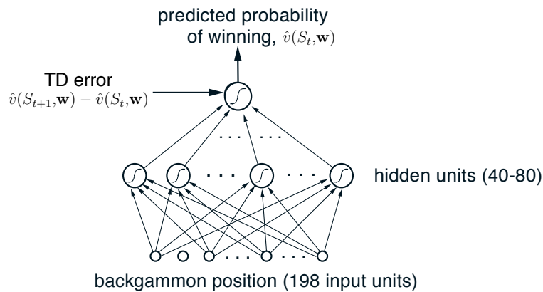
Figure 16.2: The neural network used in TD-Gammon
