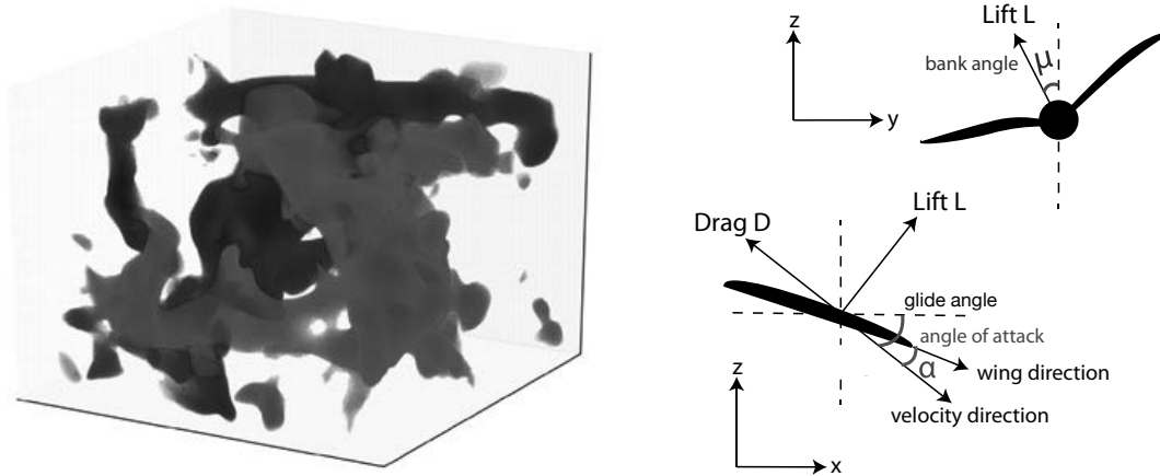
Figure 16.14: Thermal soaring model: Left: snapshot of the vertical velocity field of the simulated cube of air: in light (dark) grey is a region of large upward (downward) flow. Right: diagram of powerless flight showing bank angle \mu and angle of attack \alpha . Adapted with permission From PNAS vol. 113(22), p. E4879, 2016, Reddy, Celani, Sejnowski, and Vergassola, Learning to Soar in Turbulent Environments.
