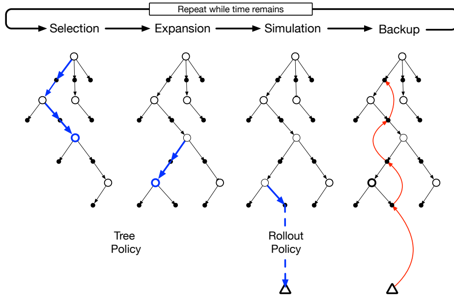
Figure 8.13: Monte Carlo Tree Search. When the environment changes to a new state, MCTS executes as many iterations as possible before an action needs to be selected, incrementally building a tree whose root node represents the current state. Each iteration consists of the four operations Selection , Expansion (though possibly skipped on some iterations), Simulation , and Backup , as explained in the text and illustrated by the bold arrows in the trees.
