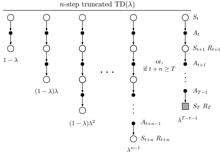
Figure 12.7: The backup diagram for truncated TD( \lambda ).
