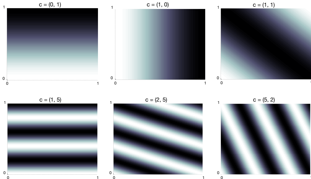
Figure 9.4: A selection of six two-dimensional Fourier cosine basis functions, each labeled by the vector c^i that defines it ( s_1 is the horizontal axis, and c^i is shown as a row vector with the index i omitted). After Konidaris et al. (2011).
