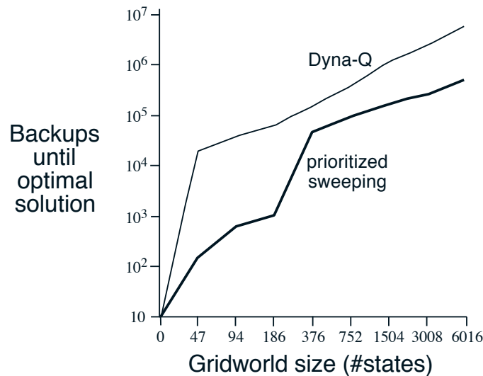
Figure 8.7: Prioritized sweeping significantly shortens learning time on the Dyna maze task for a wide range of grid resolutions. Reprinted from Peng and Williams (1993). ■
