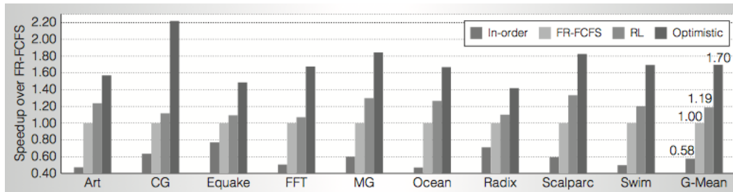
Figure 16.9: Performances of four controllers over a suite of 9 simulated benchmark applications. The controllers are: the simplest ‘in-order’ controller, FR-FCFS, the learning controller RL, and the unrealizable Optimistic controller which ignores all timing and resource constraints to provide a performance upper bound. Performance, normalized to that of FR-FCFS, is the inverse of execution time. At far right is the geometric mean of performances over the 9 benchmark applications for each controller. Controller RL comes closest to the ideal performance. ©2009 IEEE. Reprinted, with permission, from J. F. Martínez and E. İpek, Dynamic multicore resource management: A machine learning approach , Micro, IEEE , 29(5), p. 13.
