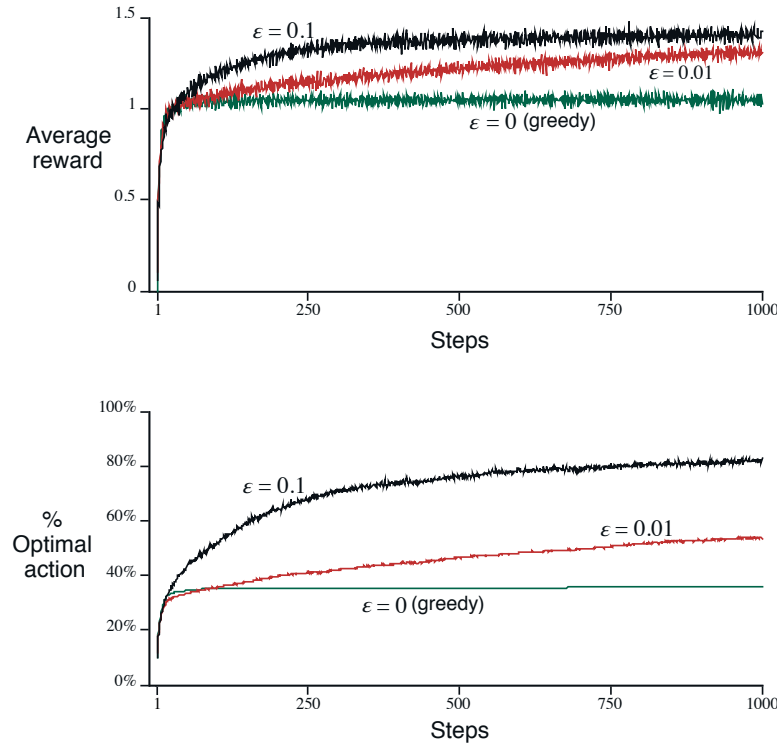
Figure 2.2: Average performance of \varepsilon -greedy action-value methods on the 10-armed testbed. These data are averages over 2000 runs with different bandit problem. All methods used sample averages as their action-value estimates.
