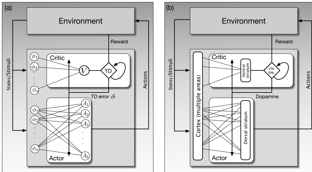
Figure 15.6: Actor-critic artificial neural network and a hypothetical neural implementation. a) Actor-critic algorithm as an artificial neural network. The actor adjusts a policy based on the TD error \delta it receives from the critic; the critic adjusts state-value parameters using the same \delta . The critic produces a TD error from the reward signal, R , and the current change in its estimate of state values. The actor does not have direct access to the reward signal, and the critic does not have direct access to the action. b) Hypothetical neural implementation of an actor-critic algorithm. The actor and the value-learning part of the critic are respectively placed in the ventral and dorsal subdivisions of the striatum. The TD error is transmitted by dopamine neurons located in the VTA and SNpc to modulate changes in synaptic efficacies of input from cortical areas to the ventral and dorsal striatum. Adapted from Frontiers in Neuroscience , vol. 2(1), 2008, Y. Takahashi, G. Schoenbaum, and Y. Niv, Silencing the critics: Understanding the effects of cocaine sensitization on dorsolateral and ventral striatum in the context of an Actor/Critic model.
