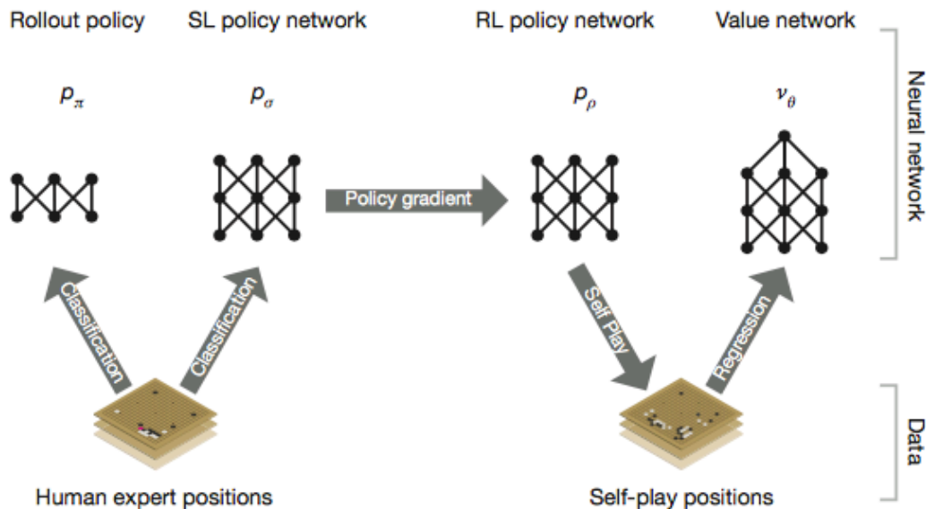
Figure 16.12: AlphaGo pipeline. Adapted with permission from Macmillan Publishers Ltd: Nature , vol. 529(7587), p. 485, copyright (2016).
