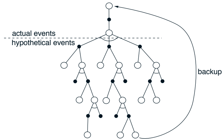
Figure 16.3: The backup diagram for Samuel's checkers player.
