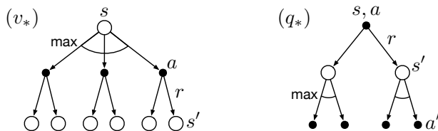
Figure 3.7: Backup diagrams for v_* and q_*
