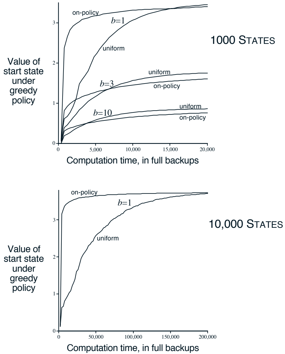
Figure 8.11: Relative efficiency of backups distributed uniformly across the state space versus focused on simulated on-policy trajectories, each starting in the same state. Results are for randomly generated tasks of two sizes and various branching factors, b .
