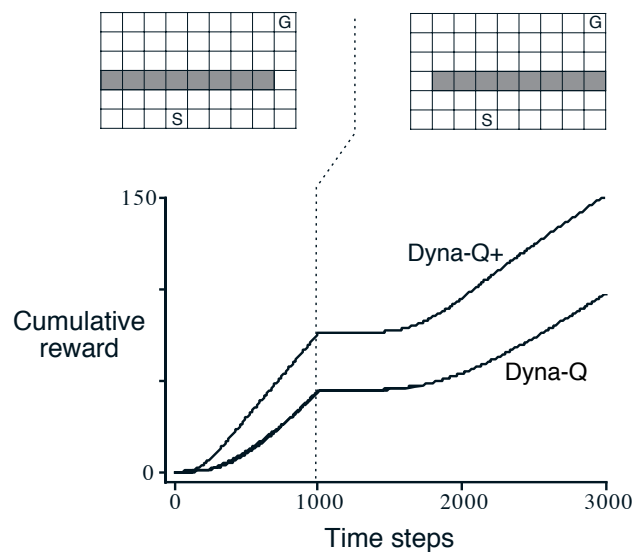
Figure 8.5: Average performance of Dyna agents on a blocking task. The left environment was used for the first 1000 steps, the right environment for the rest. Dyna-Q+ is Dyna-Q with an exploration bonus that encourages exploration. ■
