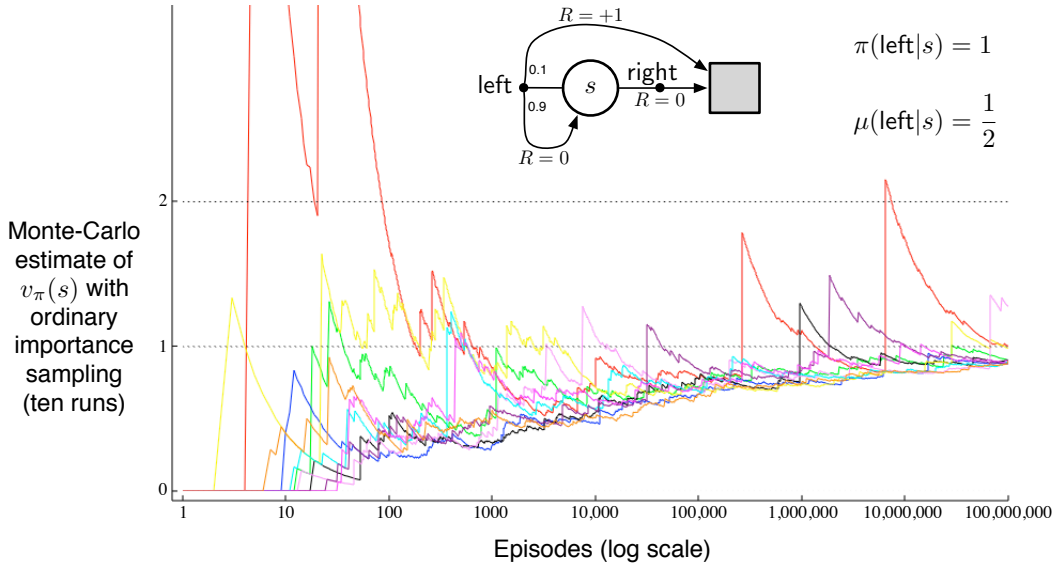
Figure 5.5: Ordinary importance sampling produces surprisingly unstable estimates on the one-state MDP shown inset (Example 5.5). The correct estimate here is 1 ( \gamma = 1 ), and, even though this is the expected value of a sample return (after importance sampling), the variance of the samples is infinite, and the estimates do not convergence to this value. These results are for off-policy first-visit MC.
