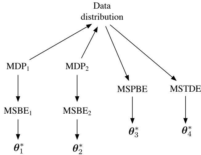
Figure 11.5: Causal relationships among the data distribution, MDPs, and errors for bootstrapping objectives. Two different MDPs can produce the same data distribution yet also produce different MSBEs and have different minimizing parameter vectors; these are not learnable from the data distribution. The MSPBE and MSTDE objectives and their (different) minima can be directly determined from data and thus are learnable.
