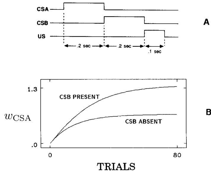
Figure 14.3: Facilitation of a remote association by an intervening stimulus in the TD model. Top: temporal relationships among stimuli within a trial. Bottom: behavior over trials of CSA's associative strength when CSA is presented in a serial compound as shown in the top panel, and when presented in an identical temporal relationship to the US, only without CSB. Adapted from Sutton and Barto (1990).
