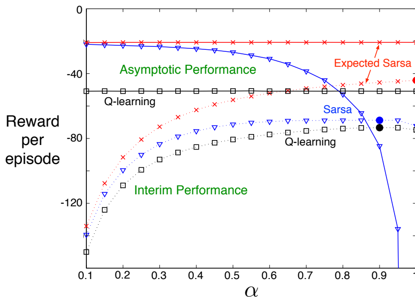
Figure 6.7: Interim and asymptotic performance of TD control methods on the cliff-walking task as a function of \alpha . All algorithms used an \varepsilon -greedy policy with \varepsilon = 0.1 . Asymptotic performance is an average over 100,000 episodes whereas interim performance is an average over the first 100 episodes. These data are averages of over 50,000 and 10 runs for the interim and asymptotic cases respectively. The solid circles mark the best interim performance of each method. Adapted from van Seijen et al. (2009).
