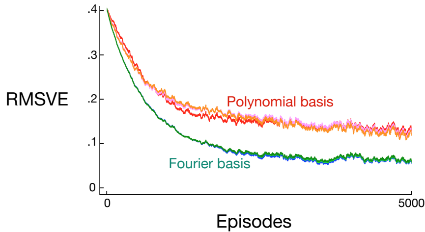
Figure 9.5: Fourier basis vs polynomials on the 1000-state random walk. Shown are learning curves for the gradient MC method with Fourier and polynomial bases of order 5, 10, and 20. The step-size parameters were roughly optimized for each case: \alpha = 0.0001 for the polynomial basis and \alpha = 0.00005 for the Fourier basis.
