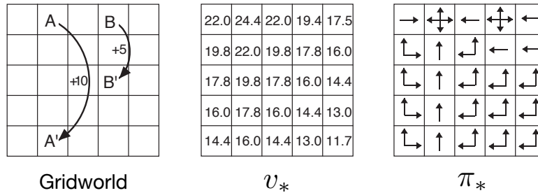
Figure 3.8: Optimal solutions to the gridworld example. ■
