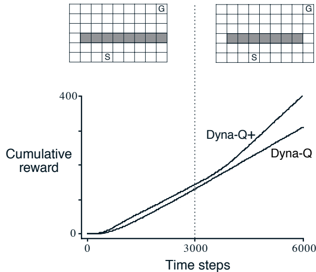
Figure 8.6: Average performance of Dyna agents on a shortcut task. The left environment was used for the first 3000 steps, the right environment for the rest. ■
