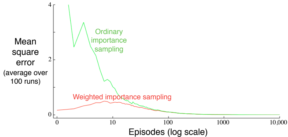
Figure 5.4: Weighted importance sampling produces lower error estimates of the value of a single blackjack state from off-policy episodes (see Example 5.4).
