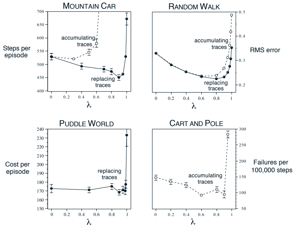
Figure 12.14: The effect of \lambda on reinforcement learning performance in four different test problems. In all cases, lower numbers represent better performance. The two left panels are applications to simple continuous-state control tasks using the Sarsa( \lambda ) algorithm and tile coding, with either replacing or accumulating traces (Sutton, 1996). The upper-right panel is for policy evaluation on a random walk task using TD( \lambda ) (Singh and Sutton, 1996). The lower right panel is unpublished data for the pole-balancing task (Example 3.4) from an earlier study (Sutton, 1984).
