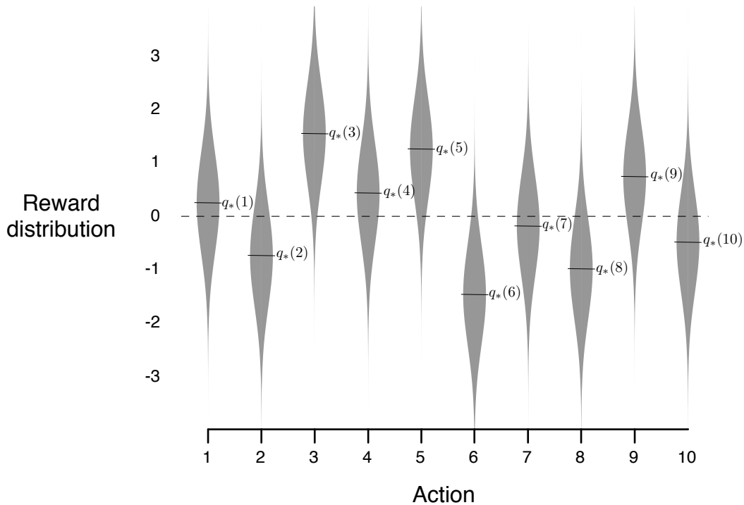
Figure 2.1: An exemplary bandit problem from the 10-armed testbed. The true value q_*(a) of each of the ten actions was selected according to a normal distribution around zero with unit variance, and then the actual rewards were selected around q_*(a) with unit variance, as suggested by these gray distributions.
