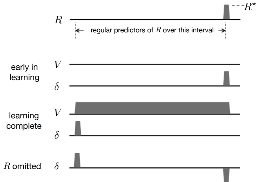
Figure 15.5: The behavior of the TD error \delta during TD learning is consistent with features of the phasic activation of dopamine neurons. (Here \delta is the TD error available at time t , i.e., \delta_{t-1} ). Top : a sequence of states, shown as an interval of regular predictors, is followed by a non-zero reward R^* . Early in learning : the initial value function, V , and initial \delta , which at first is equal to R^* . Learning complete : the value function accurately predicts future reward, \delta is positive at the earliest predictive state, and \delta = 0 at the time of the non-zero reward. R^* omitted : at the time the predicted reward is omitted, \delta becomes negative. See text for a complete explanation of why this happens.
