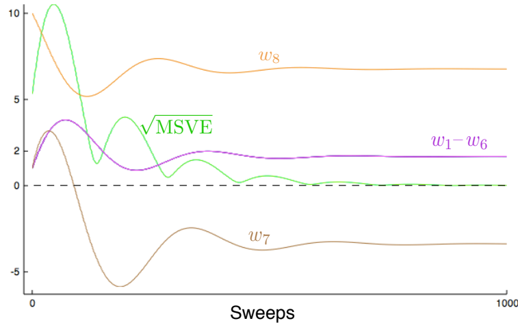
Figure 11.7: The behavior of the ETD algorithm in expectation on Baird's counterexample. The step size was \alpha = 0.03 .
