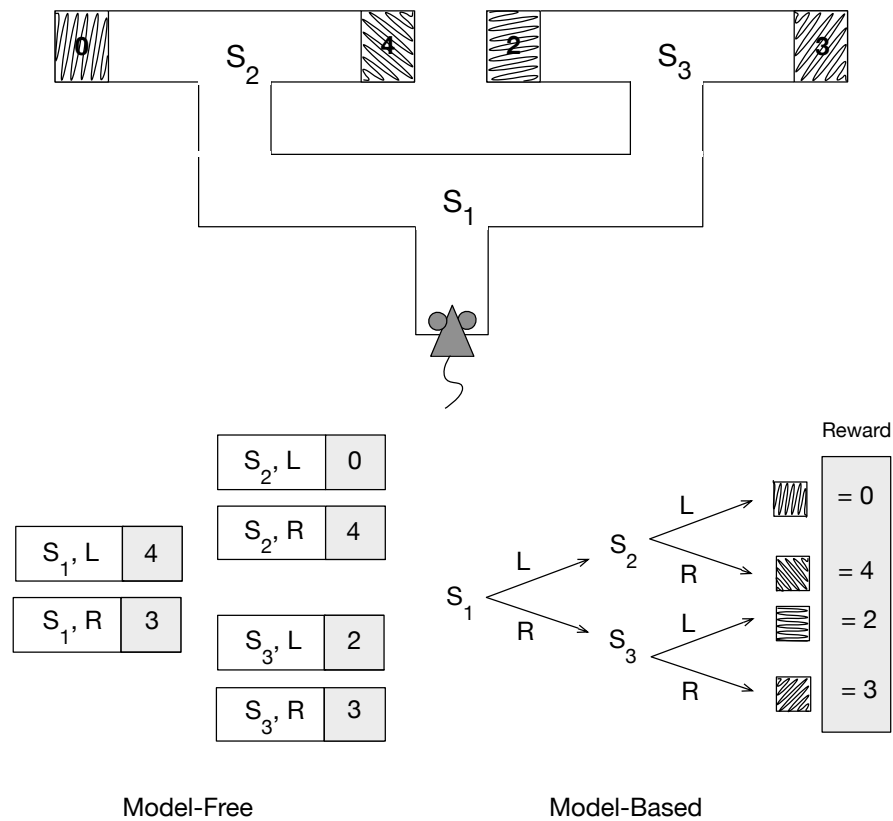
Figure 14.9: Model-based and model-free strategies to solve a hypothetical sequential action-selection problem. Top: a rat navigates a maze with distinctive goal boxes, each associated with a reward having the value shown. Lower left: a model-free strategy relies on stored action values for all the state–action pairs obtained over many learning trials. To make decisions the rat just has to select at each state the action with the largest action value for that state. Lower right: in a model-based strategy, the rat learns an environment model, consisting of knowledge of state–action–next-state transitions and a reward model consisting of knowledge of the reward associated with each distinctive goal box. The rat can decide which way to turn at each state by using the model to simulate sequences of action choices to find a path yielding the highest return. Adapted from Trends in Cognitive Science , volume 10, number 8, Y. Niv, D. Joel, and P. Dayan, A Normative Perspective on Motivation, p. 376, 2006, with permission from Elsevier.
