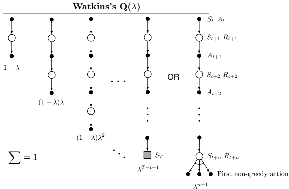
Figure 12.12: The backup diagram for Watkins's Q(\lambda) . The series of component backups ends either with the end of the episode or with the first nongreedy action, whichever comes first.
