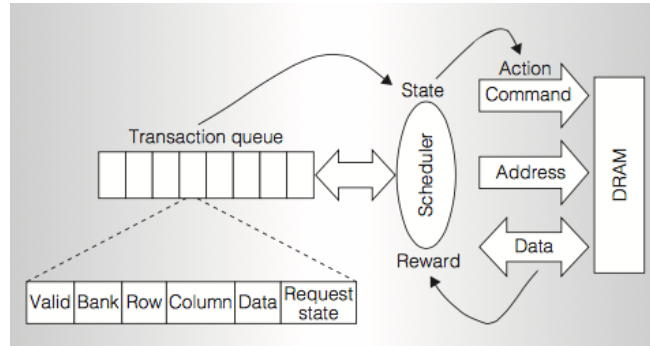
Figure 16.8: High-level view of the reinforcement learning DRAM controller. The scheduler is the reinforcement learning agent. Its environment is represented by features of the transaction queue, and its actions are commands to the DRAM system. ©2009 IEEE. Reprinted, with permission, from J. F. Martínez and E. İpek, Dynamic multicore resource management: A machine learning approach, Micro , IEEE, 29(5), p. 12.
