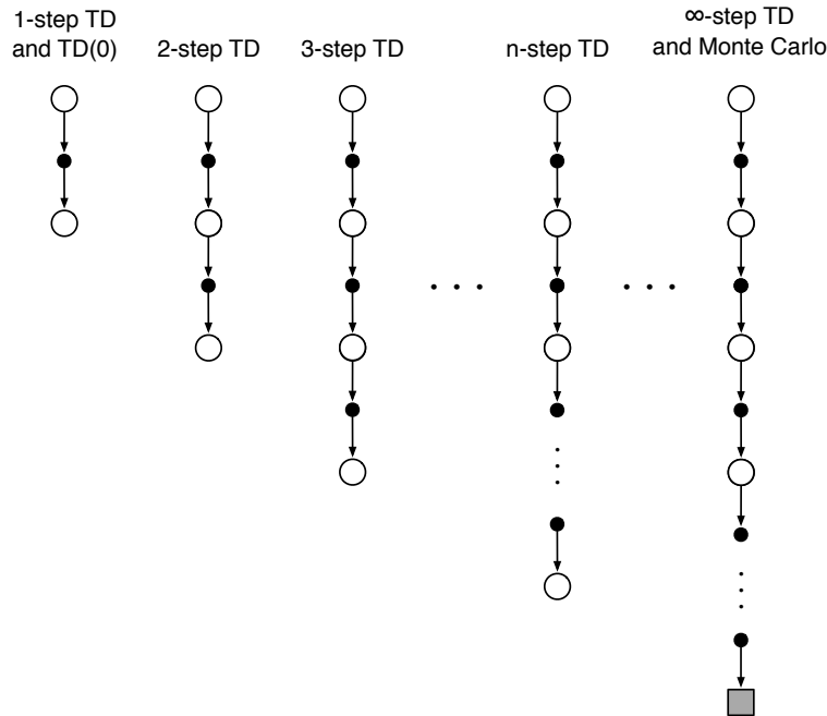
Figure 7.1: The spectrum ranging from the one-step backups of simple TD methods to the up-until-termination backups of Monte Carlo methods. In between are the n -step backups, based on n steps of real rewards and the estimated value of the n th next state, all appropriately discounted.
