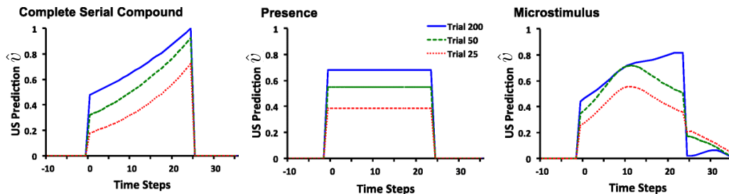
Figure 14.7: Time course of US prediction over the course of acquisition for the TD model with three different stimulus representations. Left: With the complete serial compound (CSC), the US prediction increases exponentially through the interval, peaking at the time of the US. At asymptote (trial 200), the US prediction peaks at the US intensity (1 in these simulations). Middle: With the presence representation, the US prediction converges to an almost constant level. This constant level is determined by the US intensity and the length of the CS–US interval. Right: With the microstimulus representation, at asymptote, the TD model approximates the exponentially increasing time course depicted with the CSC through a linear combination of the different microstimuli. Adapted with minor changes from Learning & Behavior , Evaluating the TD Model of Classical Conditioning, volume 40, 2012, E. A. Ludvig, R. S. Sutton, E. J. Kehoe. With permission of Springer.
