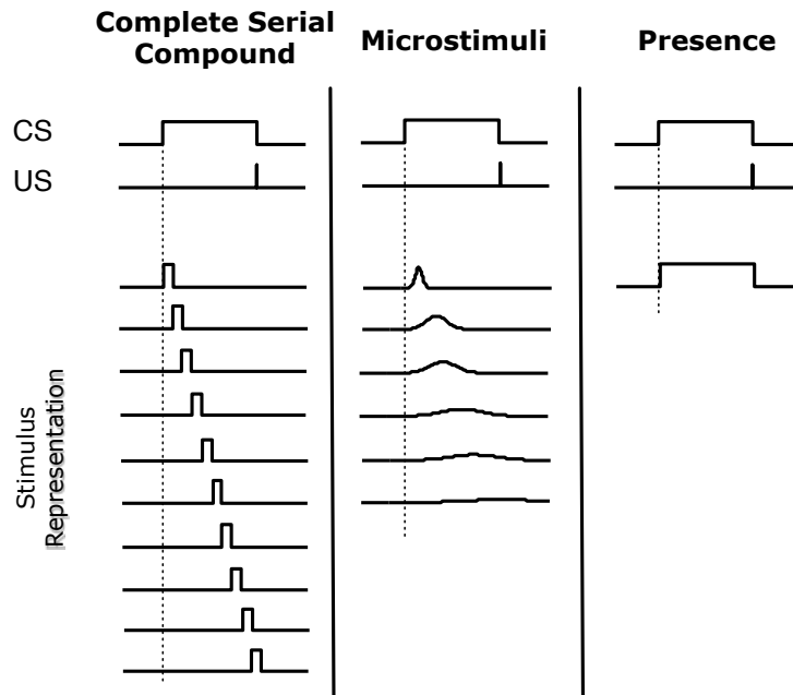
Figure 14.2: Three stimulus representations (in columns) sometimes used with the TD model. Each row represents one element of the stimulus representation. The three representations vary along a temporal generalization gradient, with no generalization between nearby time points in the complete serial compound (left column) and complete generalization between nearby time points in the presence representation (right column). The microstimulus representation occupies a middle ground. The degree of temporal generalization determines the temporal granularity with which US predictions are learned. Adapted with minor changes from Learning & Behavior , Evaluating the TD Model of Classical Conditioning, volume 40, 2012, p. 311, E. A. Ludvig, R. S. Sutton, E. J. Kehoe. With permission of Springer.
