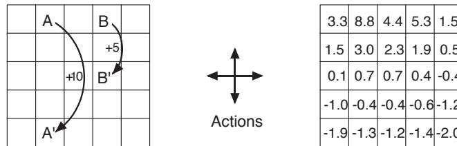
Figure 3.5: Gridworld example: exceptional reward dynamics (left) and state-value function for the equiprobable random policy (right).
