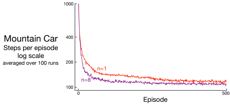
Figure 10.3: One-step vs multi-step performance of n -step semi-gradient Sarsa on the Mountain Car task. Good step sizes were used: \alpha = 0.5/8 for n = 1 and \alpha = 0.3/8 for n = 8 .
