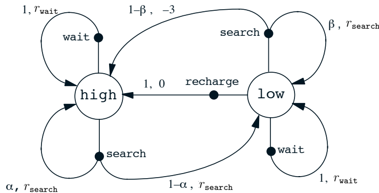
Figure 3.3: Transition graph for the recycling robot example.
