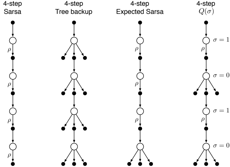
Figure 7.5: The three kinds of n -step action-value backups considered so far in this chapter (4-step case) plus a fourth kind of backup that unifies them all. The ‘ \rho ’s indicate half transitions on which importance sampling is required in the off-policy case. The fourth kind of backup unifies all the others by choosing on a state-by-state basis whether to sample ( \sigma_t = 1 ) or not ( \sigma_t = 0 ).
