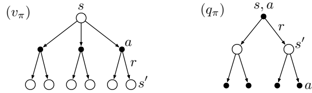
Figure 3.4: Backup diagrams for v_\pi and q_\pi .
