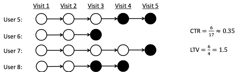
Figure 16.13: Click through rate (CTR) versus life-time value (LTV). Each circle represents a user visit; black circles are visits at which the user clicks. Adapted from Theocharous et al. (2015) permission pending.
