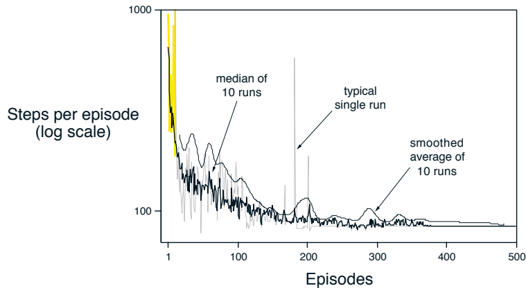
Figure 16.6: Learning curves for Sarsa( \lambda ) on the acrobot task.
