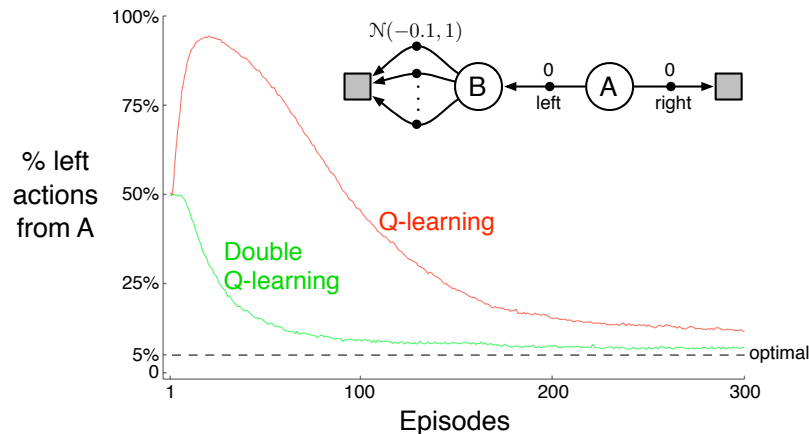
Figure 6.8: Comparison of Q-learning and Double Q-learning on a simple episodic MDP (shown inset). Q-learning initially learns to take the left action much more often than the right action, and always takes it significantly more often than the 5% minimum probability enforced by \epsilon -greedy action selection with \epsilon = 0.1 . In contrast, Double Q-learning is essentially unaffected by maximization bias. These data are averaged over 10,000 runs. The initial action-value estimates were zero. Any ties in \epsilon -greedy action selection were broken randomly. ■
