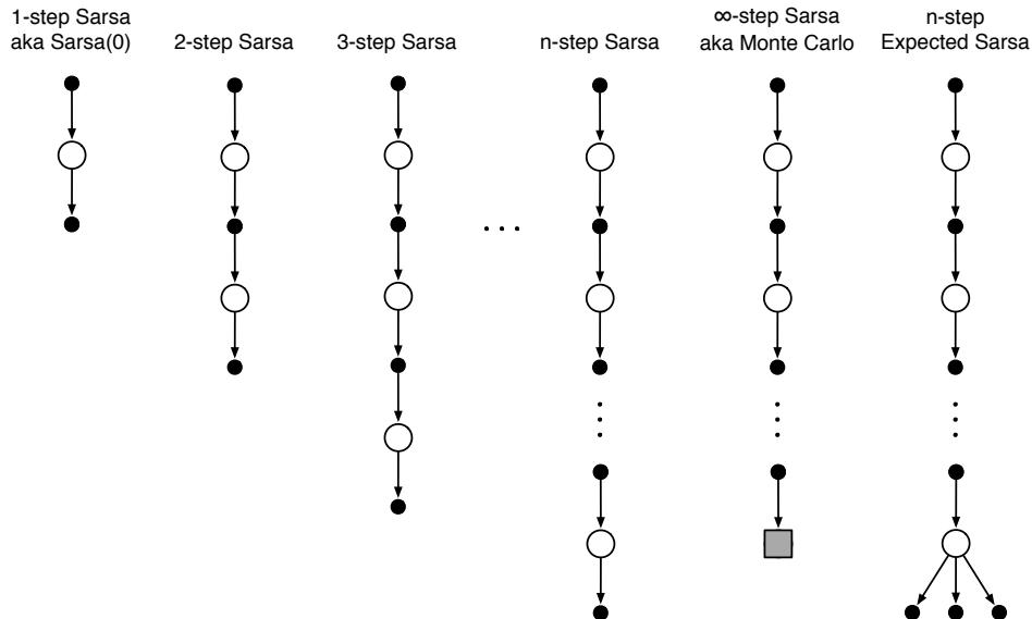
Figure 7.3: The spectrum of n -step backups for state–action values. They range from the one-step backup of Sarsa(0) to the up-until-termination backup of a Monte Carlo method. In between are the n -step backups, based on n steps of real rewards and the estimated value of the n th next state–action pair, all appropriately discounted. On the far right is the backup diagram for n -step Expected Sarsa.
