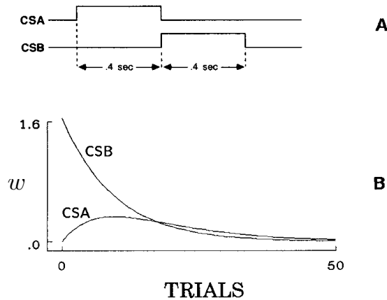
Figure 14.6: Second-order conditioning with the TD model. Top: temporal relationships between stimuli. Bottom: behavior of the associative strengths associated with CSA and CSB over trials. The second stimulus, CSB, has an initial associative strength of 1.653 at the beginning of the simulation. Adapted from Sutton and Barto (1990).
