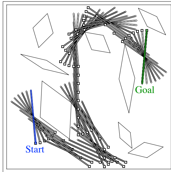
Figure 8.8: A rod-maneuvering task and its solution by prioritized sweeping. Reprinted from Moore and Atkeson (1993). ■
