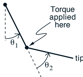
Figure 16.4: The acrobot.
