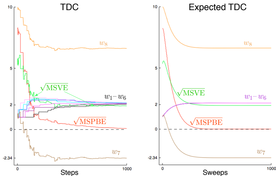
Figure 11.6: The behavior of the TDC algorithm on Baird’s counterexample. On the left is shown a typical single run, and on the right is shown the expected behavior of this algorithm if the updates are done in asynchronous sweeps (analogous to (11.7), except for the two TDC parameter vectors). The step sizes were \alpha = 0.005 and \beta = 0.05 .
