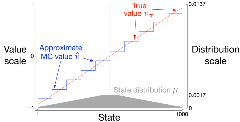
Figure 9.1: Function approximation by state aggregation on the 1000-state random walk task, using the gradient Monte Carlo algorithm (page 216).
