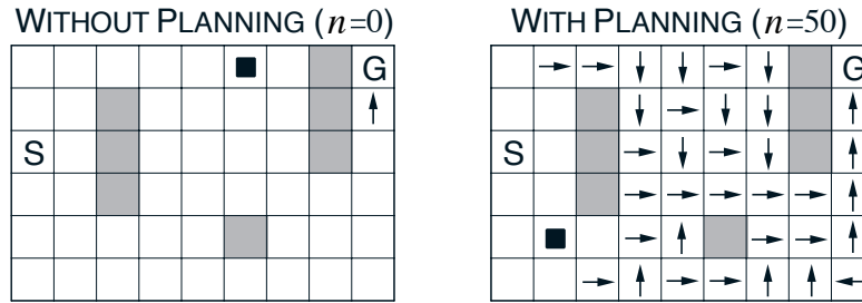
Figure 8.4: Policies found by planning and nonplanning Dyna-Q agents halfway through the second episode. The arrows indicate the greedy action in each state; if no arrow is shown for a state, then all of its action values were equal. The black square indicates the location of the agent.
