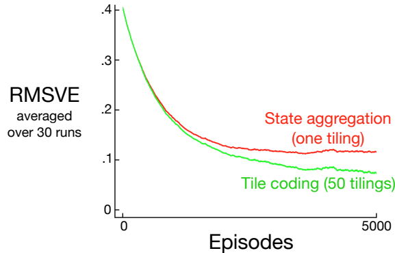
Figure 9.10: Why we use coarse coding. Shown are learning curves on the 1000-state random walk example for the gradient MC algorithm with a single tiling and with multiple tilings. The space of 1000 states was treated as a single continuous dimension, covered with tiles each 200 states wide. The multiple tilings were offset from each other by 4 states. The step-size parameter was set so that the initial learning rate in the two cases was the same, \alpha = 0.0001 for the single tiling and \alpha = 0.0001/50 for the 50 tilings.
