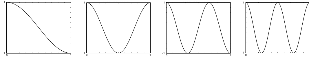
Figure 9.3: One-dimensional Fourier cosine basis functions x_i , i = 1, 2, 3, 4 , for approximating functions over the interval [0, 1] ; x_0 is a constant function. After Konidaris et al. (2011).
