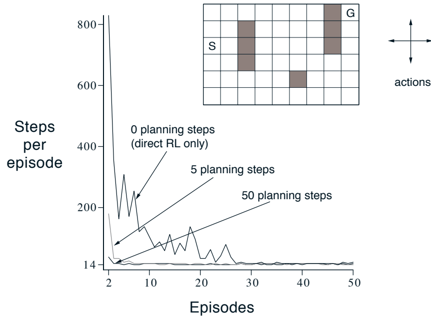
Figure 8.3: A simple maze (inset) and the average learning curves for Dyna-Q agents varying in their number of planning steps ( n ) per real step. The task is to travel from S to G as quickly as possible.
