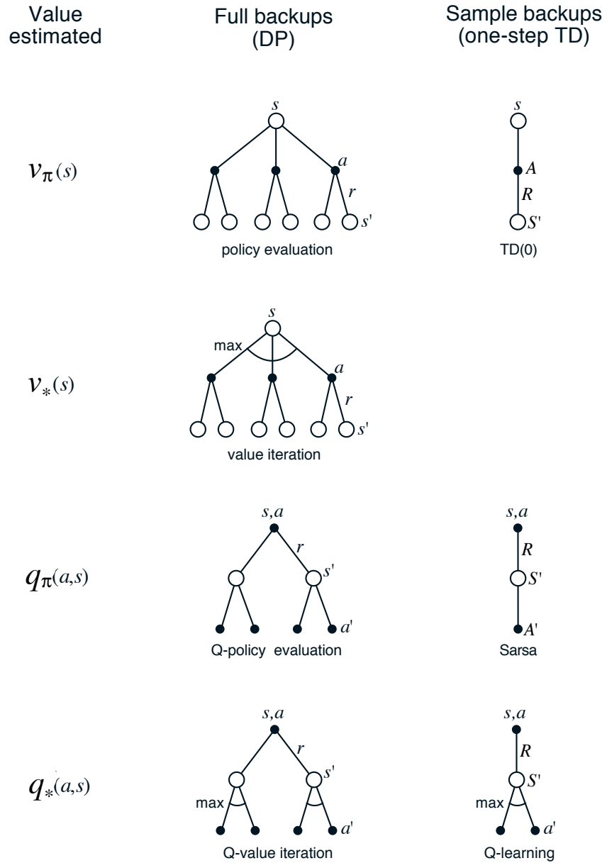
Figure 8.9: The one-step backups.
