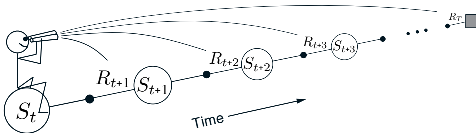
Figure 12.4: The forward view. We decide how to update each state by looking forward to future rewards and states.
