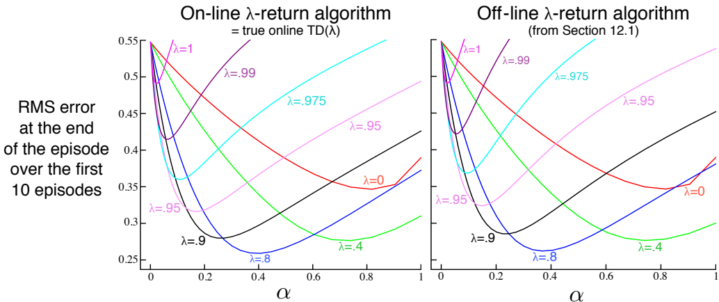
Figure 12.8: 19-state Random walk results (Example 7.1): Performance of online and off-line \lambda -return algorithms. The performance measure here is the \sqrt{\text{VE}} at the end of the episode, which should be the best case for the off-line algorithm. Nevertheless, the online algorithm performs subtly better. For comparison, the \lambda=0 line is the same for both methods.
