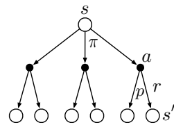
Backup diagram for v_\pi
