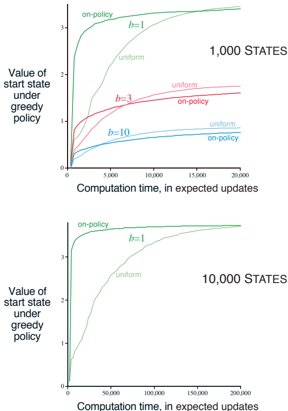
Figure 8.8: Relative efficiency of updates distributed uniformly across the state space versus focus on simulated on-policy trajectories, each starting in the same state. Results are for randomly generated tasks of two sizes and various branching factors, b .
