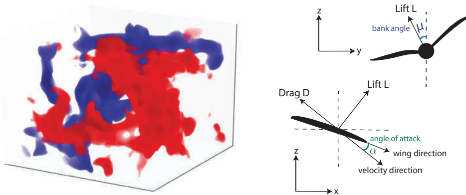
Figure 16.9: Thermal soaring model: Left: snapshot of the vertical velocity field of the simulated cube of air: in red (blue) is a region of large upward (downward) flow. Right: diagram of powerless flight showing bank angle \mu and angle of attack \alpha . Adapted with permission From PNAS vol. 113(22), p. E4879, 2016, Reddy, Celani, Sejnowski, and Vergassola, Learning to Soar in Turbulent Environments.
