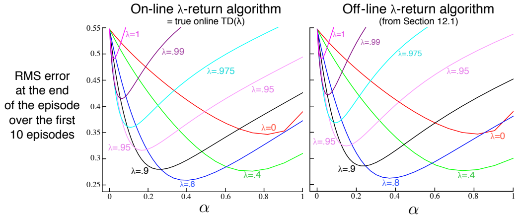
Figure 12.8: 19-state Random walk results (Example 7.1): Performance of online and off-line \lambda -return algorithms. The performance measure here is the \overline{VE} at the end of the episode, which should be the best case for the off-line algorithm. Nevertheless, the online algorithm performs subtly better. For comparison, the \lambda=0 line is the same for both methods.
